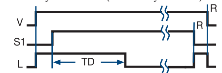
Delay-on-Make (Normally Closed)
